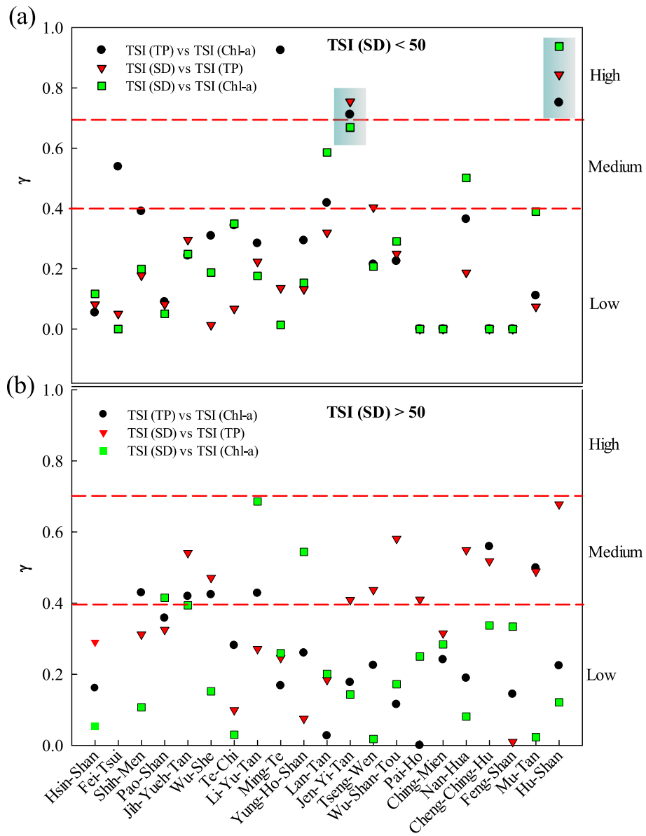
Fig. 8 Pearson correlation between TSI variables at the condition of (a) TSI (SD) < 50 and (b) TSI (SD) > 50
