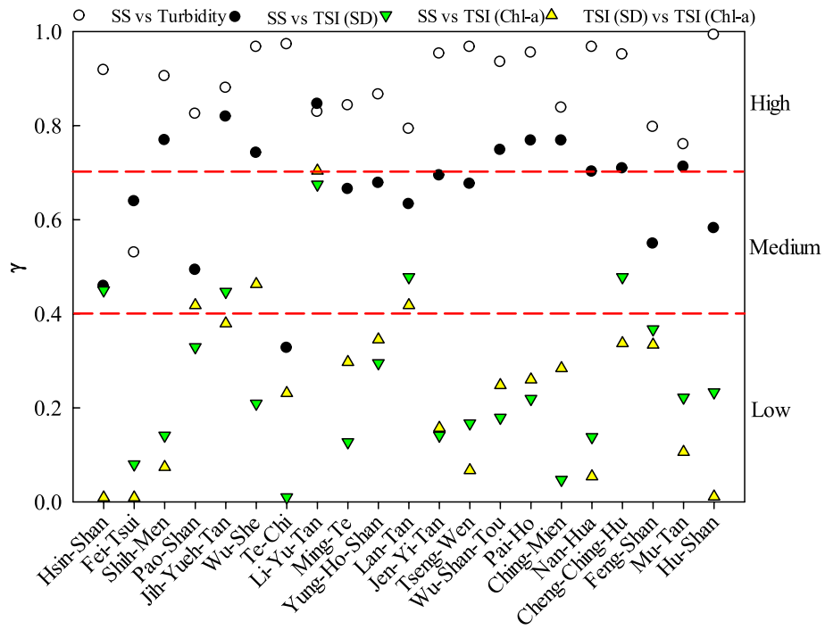
Fig. 7 Pearson correlation coefficient for SS, turbidity, TSI (SD), and TSI (Chl-a)
